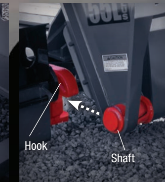
2. As the gooseneck approaches the deck, the Shaft on the gooseneck slides under the Hook on the deck
