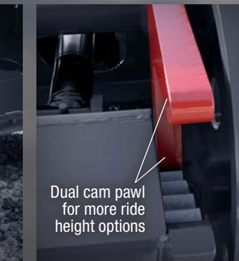
4. The dual cam pawl (now standard on hydraulic gooseneck models) gives you additional ride height options for greater flexibility
